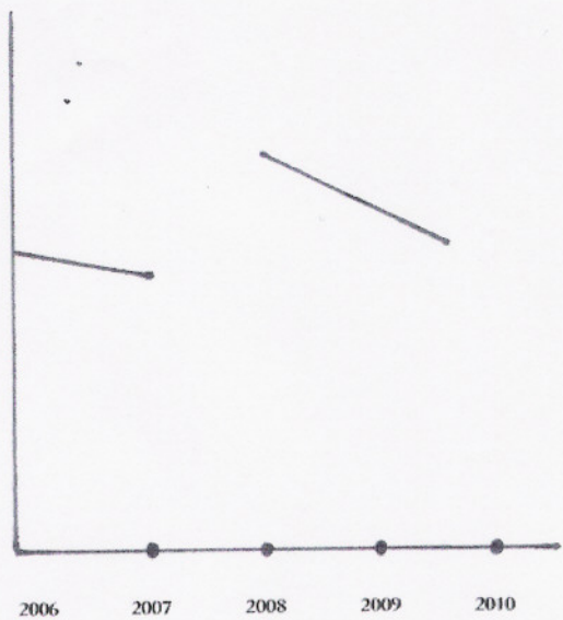
Chart 1: Crime rate
